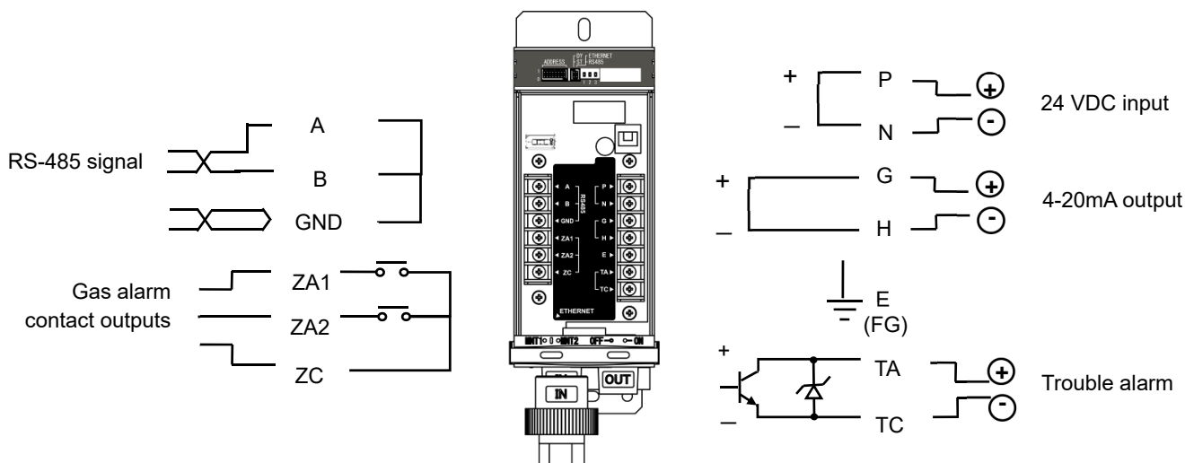
Terminal layout
