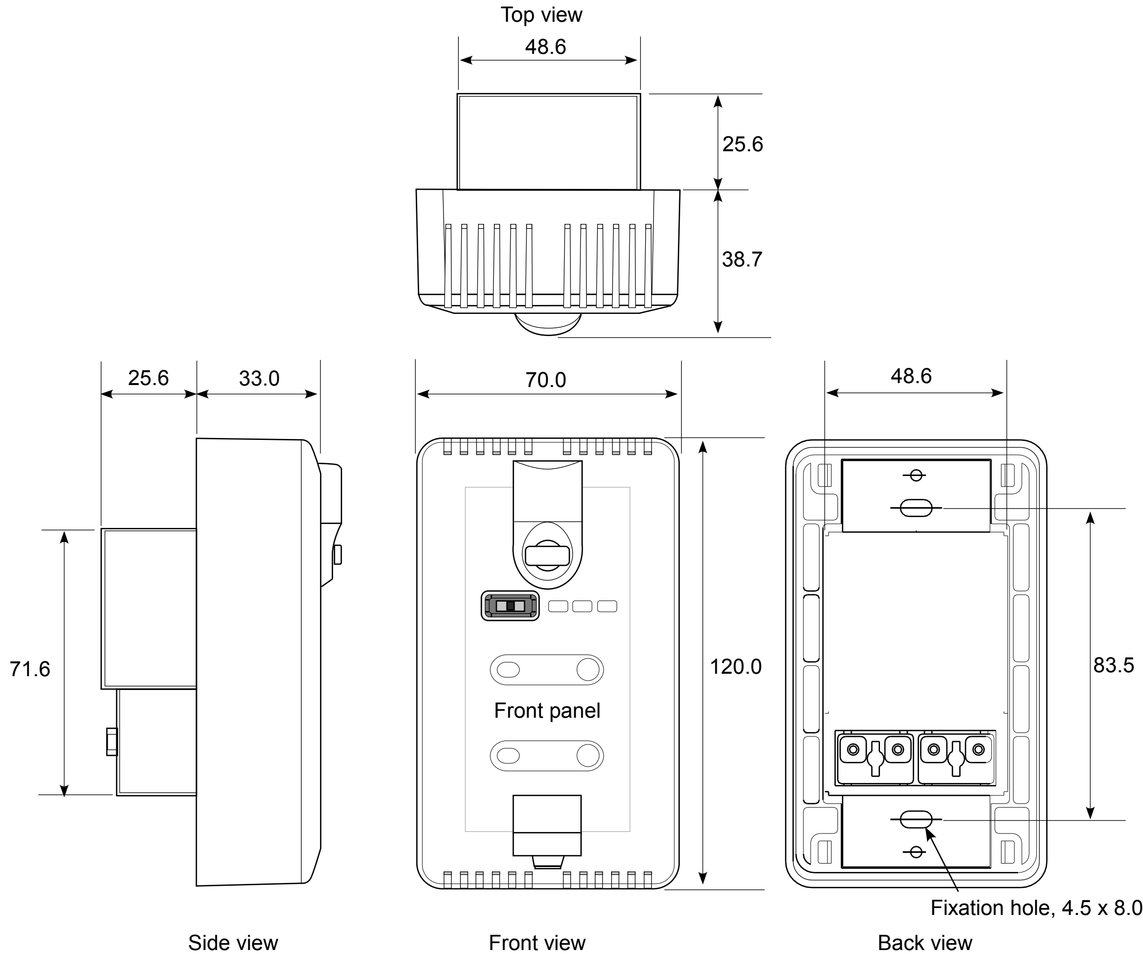
Outside drawing of ARU-03C, ARU-03S, ARU-05C, and ARU-05S
